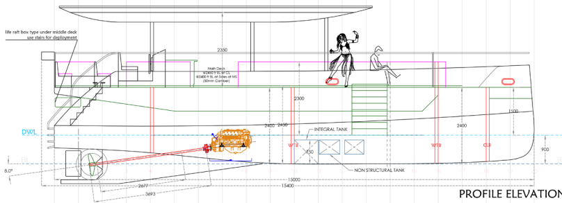
PROFILE ELEVATION
