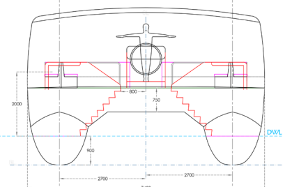
SECT. ELEVATION
