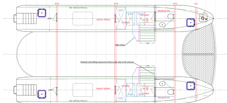
LOWER DECK
