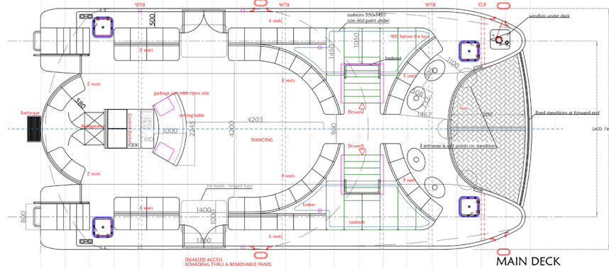
MAIN DECK
